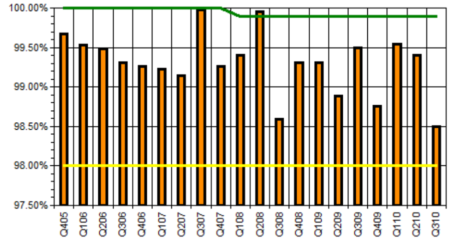
Total System Availability
