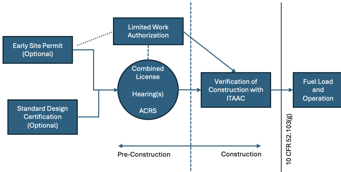
Figure 26. COLA Process [146]
