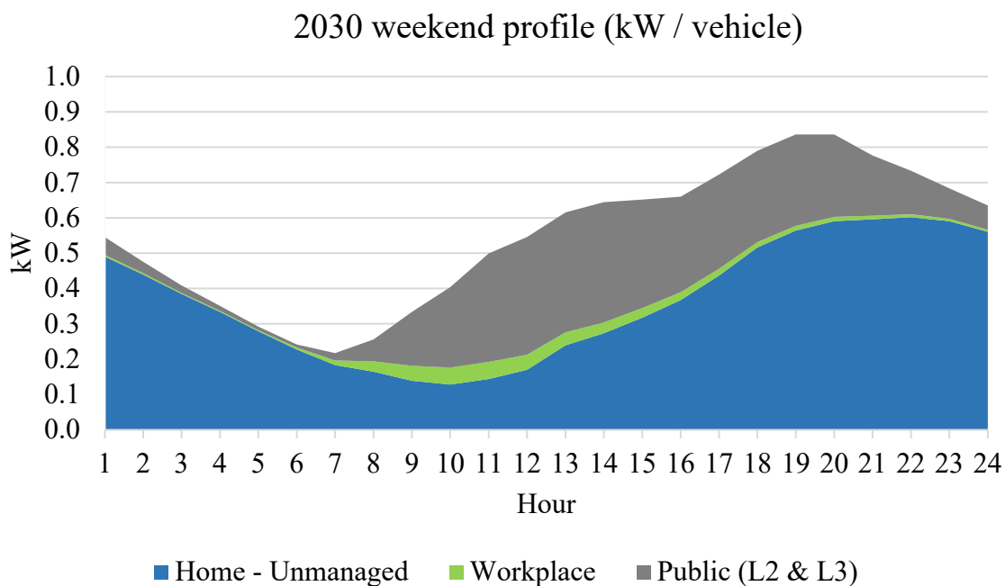
Figure 3-15: LDV EV 2030 Weekend Charging Profile (kW/vehicle)
