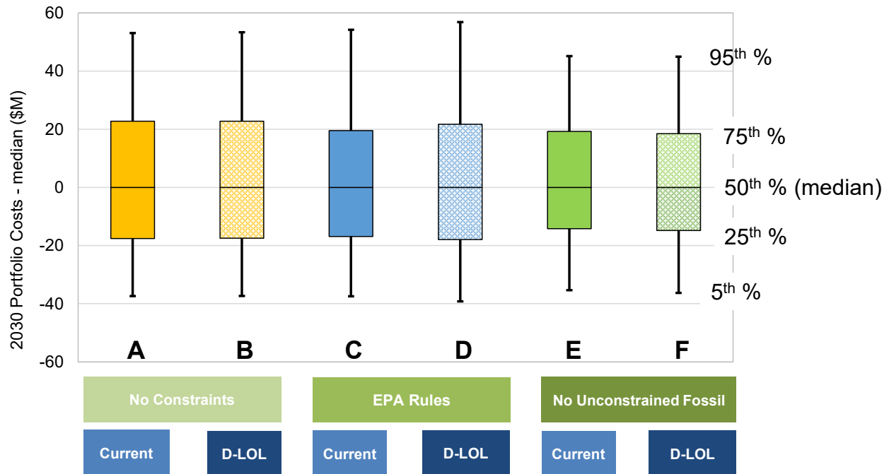
Figure 9-24: Distribution of Cost Risk across Portfolios – 2030, Normalized to the Median Cost
