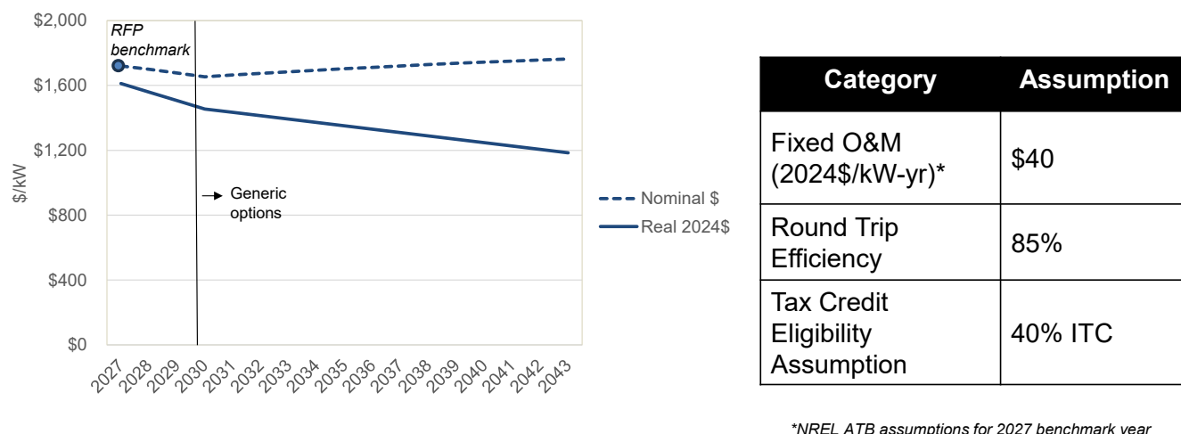
Figure 4-14: Long-Term Four-Hour Lithium-Ion Storage Cost Assumptions
