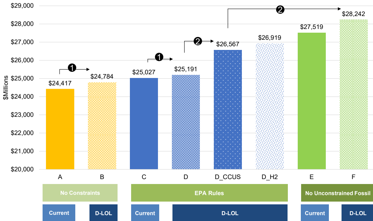
Figure 9-18: Accelerated Innovation Scenario Cost to Customer (30-year NPVRR – millions of $)
