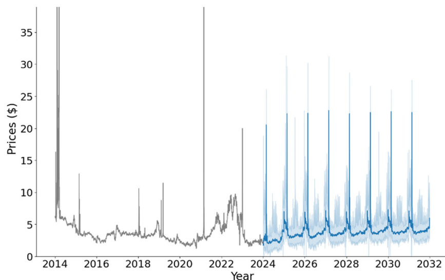
Figure 8-48: Future Natural Gas Price Iterations (Daily)
