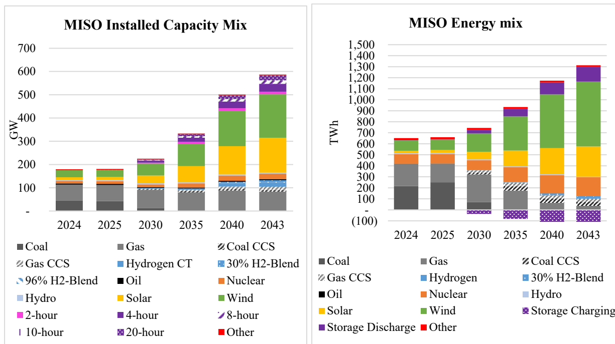
Figure 8-32: MISO Power Market Evolution for AI Scenario
