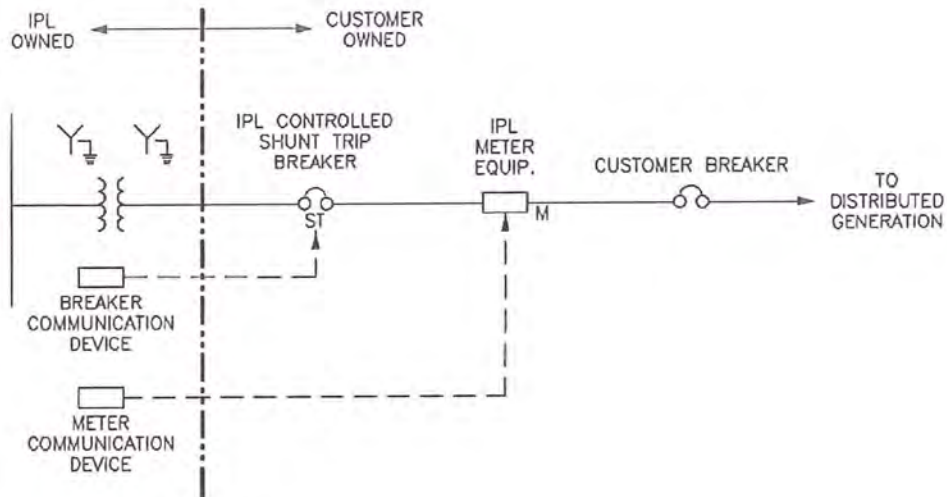
UNDERGROUND SINGLE LINE DIAGRAM
