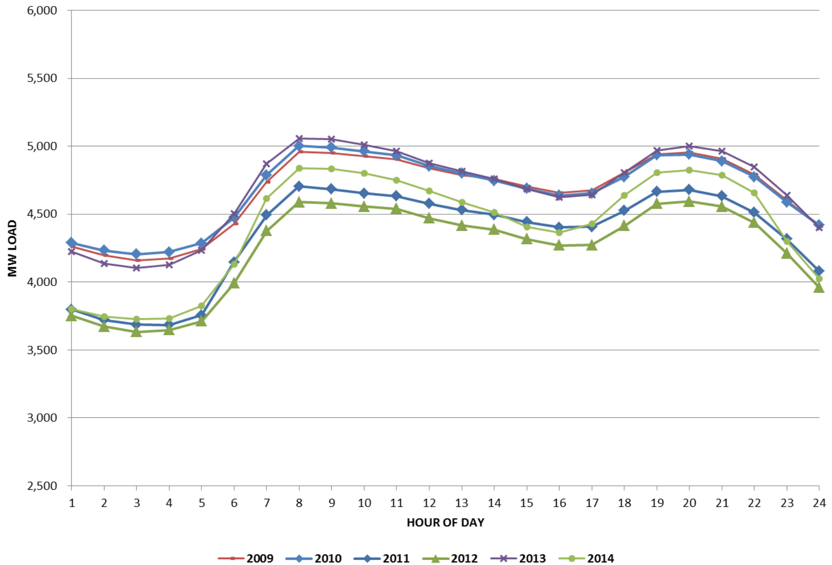
DUKE ENERGY INDIANA TYPICAL WINTER WEEKDAY 24-HOUR LOAD SHAPE, 2009-2014
