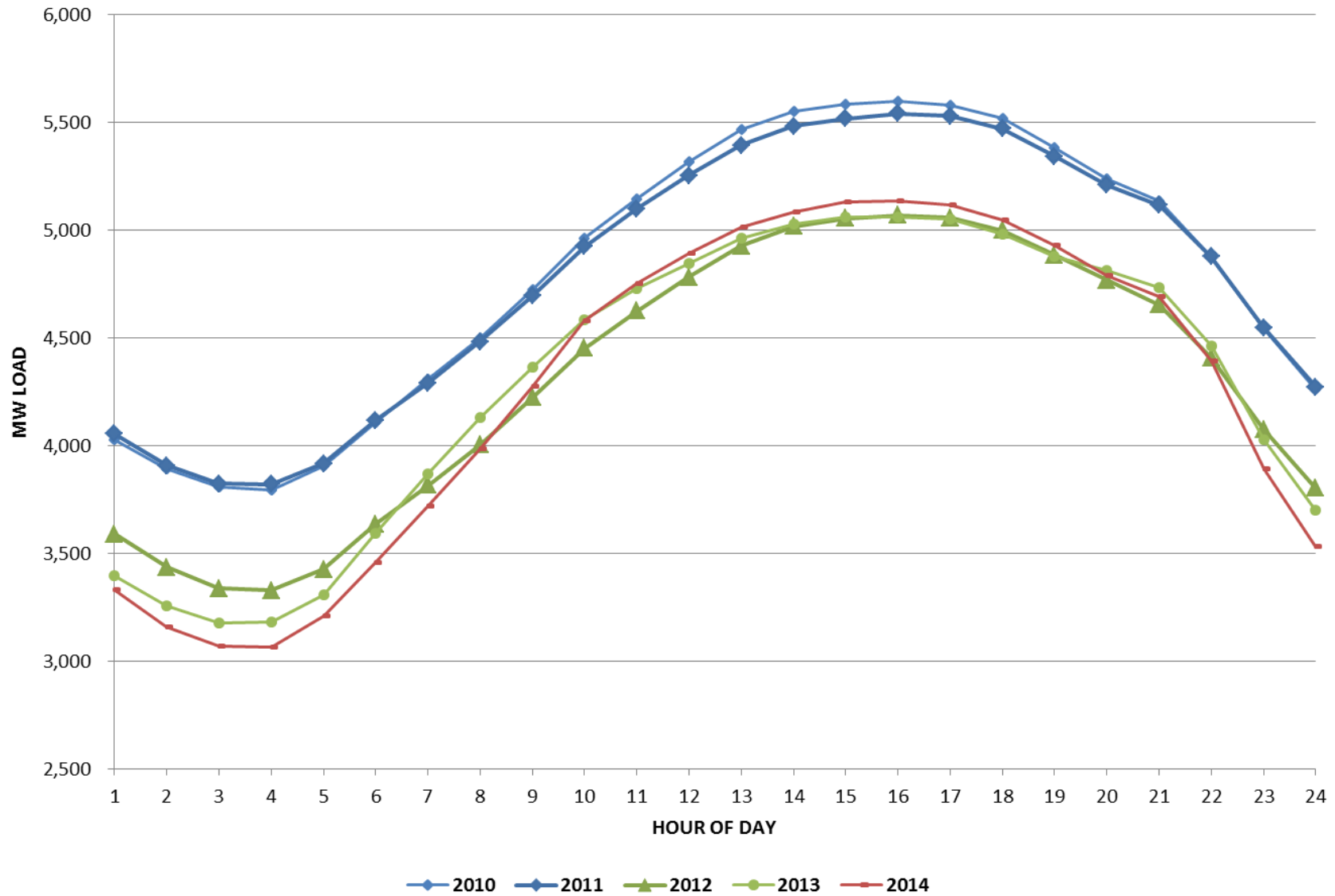
DUKE ENERGY INDIANA TYPICAL SUMMER WEEKDAY 24-HOUR LOAD SHAPE, 2010-2014
