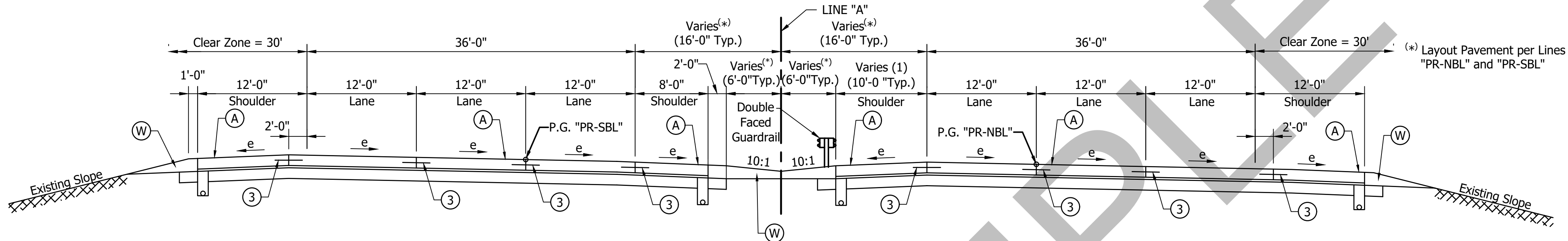
TYPICAL SUPERELEVATION SECTION
