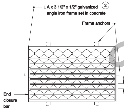
STEEL GRATING AND FRAME TYPE 12A
