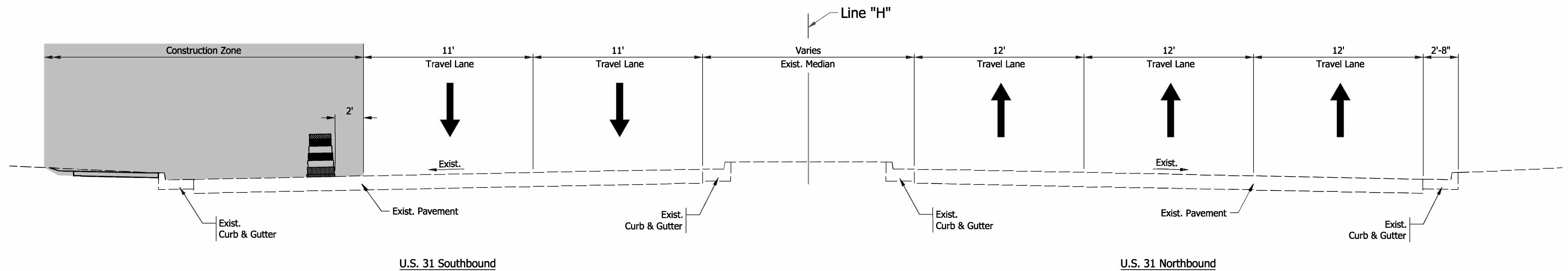
STAGE 2 MAINTENANCE OF TRAFFIC SECTION STA 690+00 TO STA 836+54
