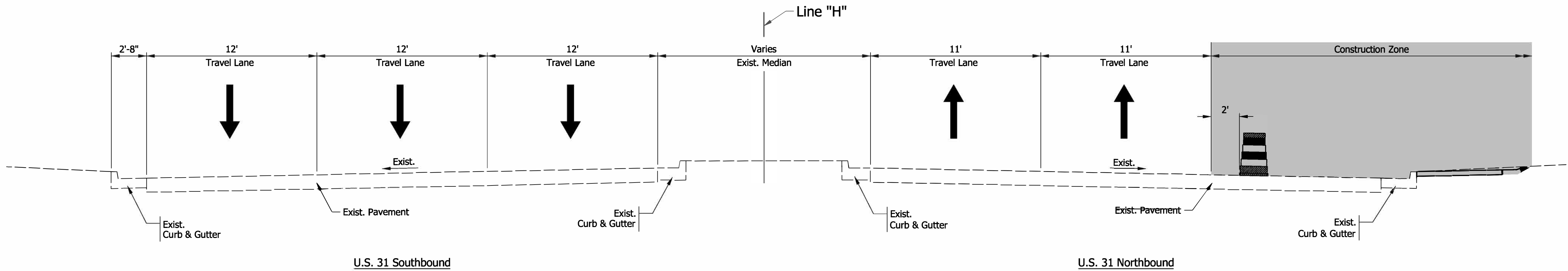
PHASE 1 MAINTENANCE OF TRAFFIC SECTION STA 693+15 TO STA 834+74
