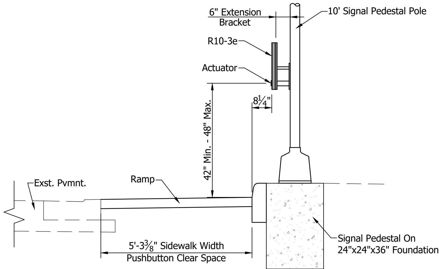
PEDESTRIAN PUSHBUTTON ASSEMBLY NE CORNER OF U.S. 31 @ SHELBY ST. (Looking North)
