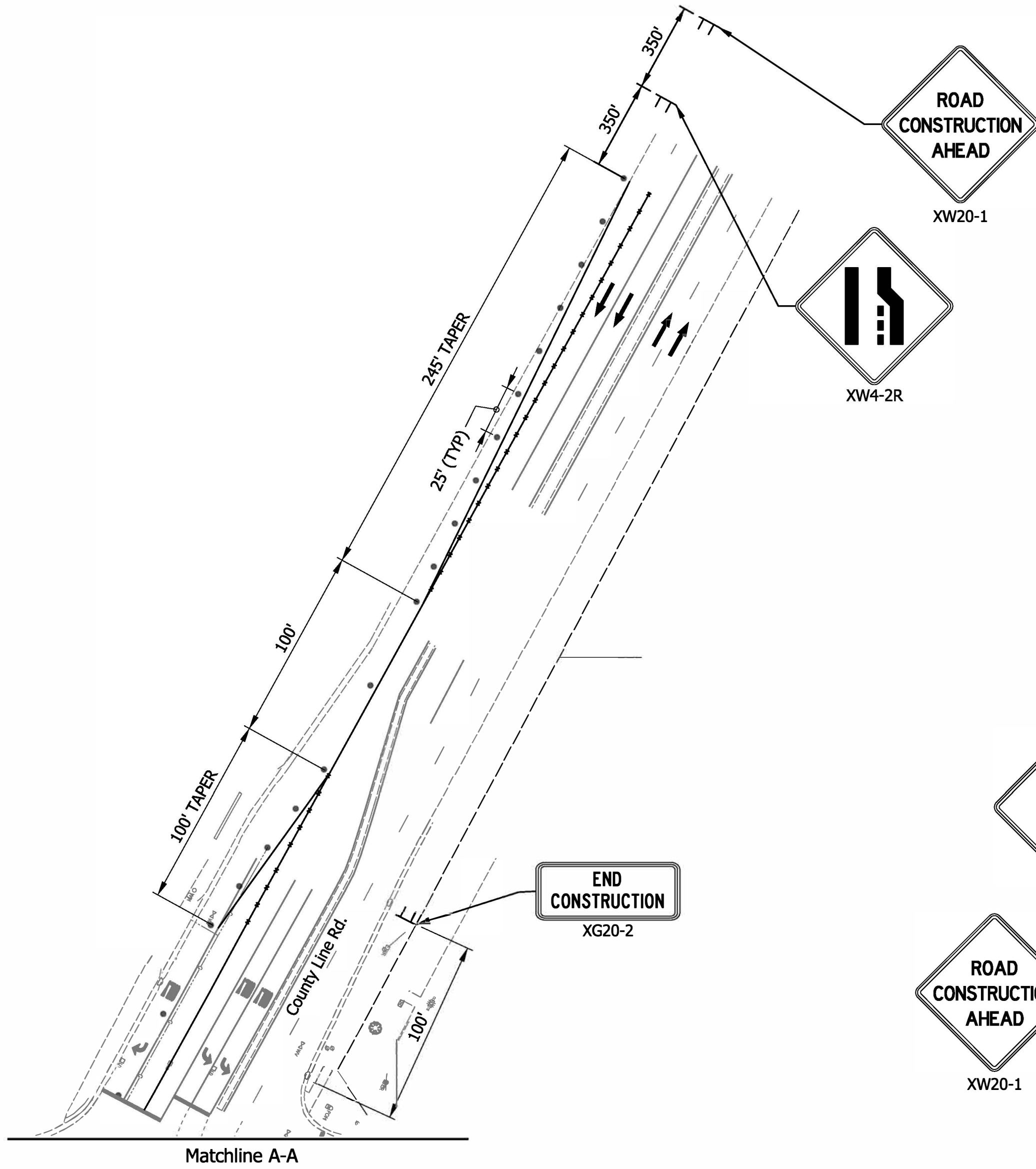
Detail C
