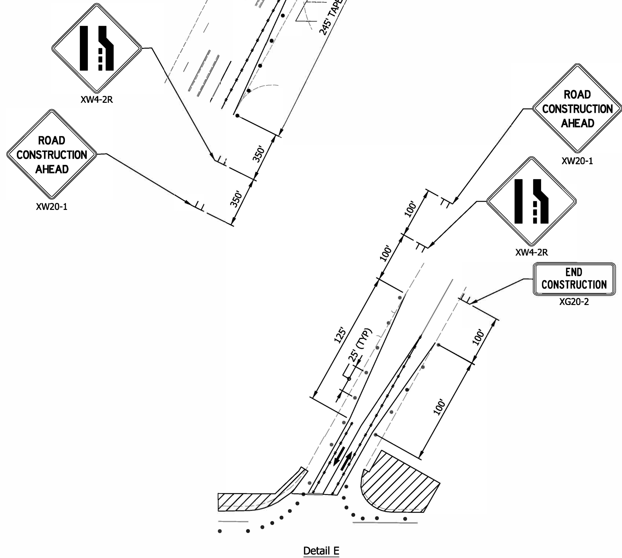
Detail E
