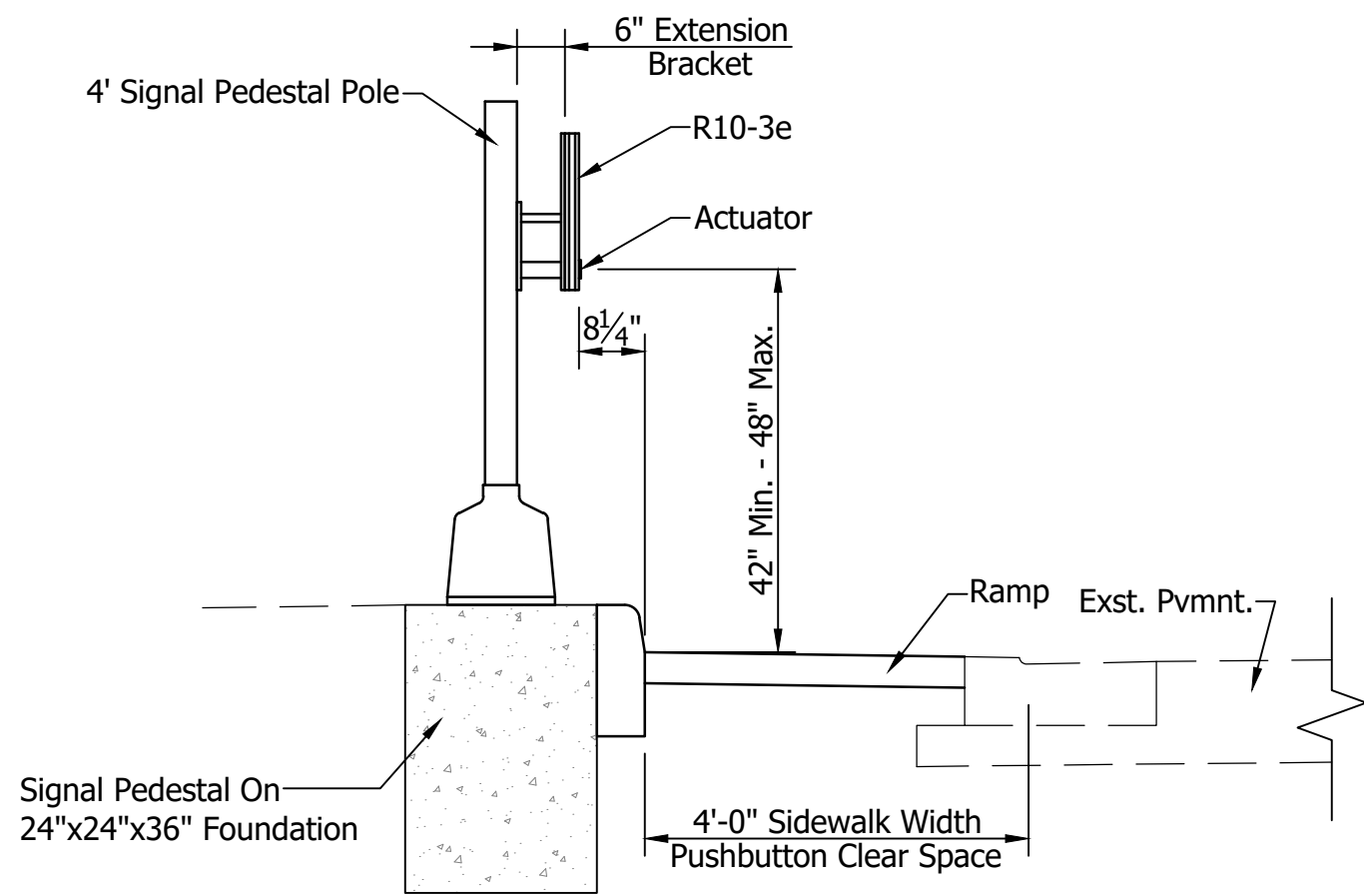
PEDESTRIAN PUSHBUTTON ASSEMBLY SE CORNER OF U.S. 31 @ SHELBY ST. (Looking South)
