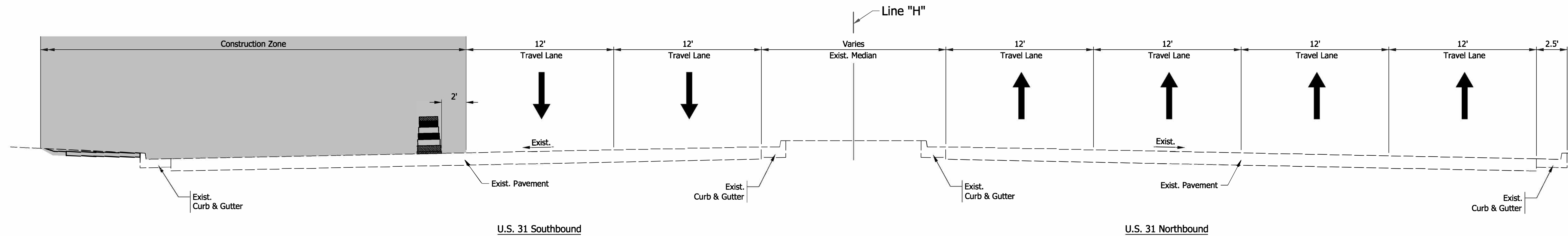
STAGE 2 MAINTENANCE OF TRAFFIC SECTION STA 610+75 TO STA 690+00
