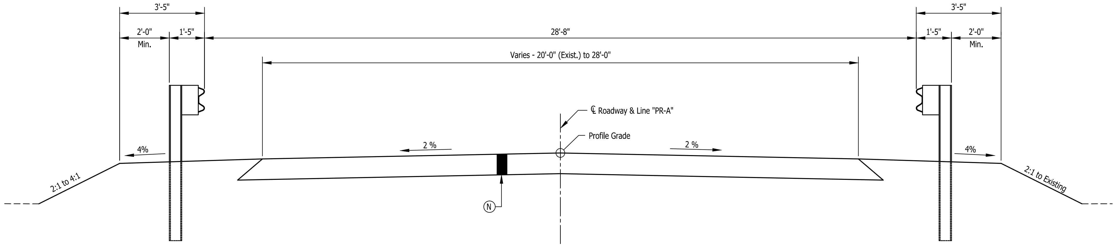
TYPICAL VARIABLE-DEPTH SECTION Sta. 25+00.49 to 25+50.83 (Varies from 28'-0" to existing)
