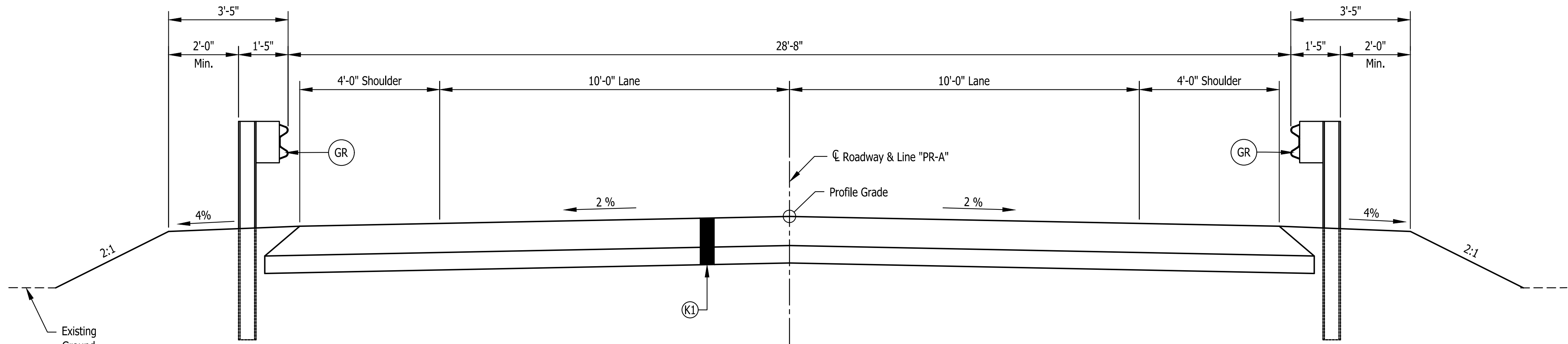
TYPICAL FULL-DEPTH SECTION Sta. 22+05.08 to Sta. 22+63.73 Sta. 24+24.85 to 25+00.49
