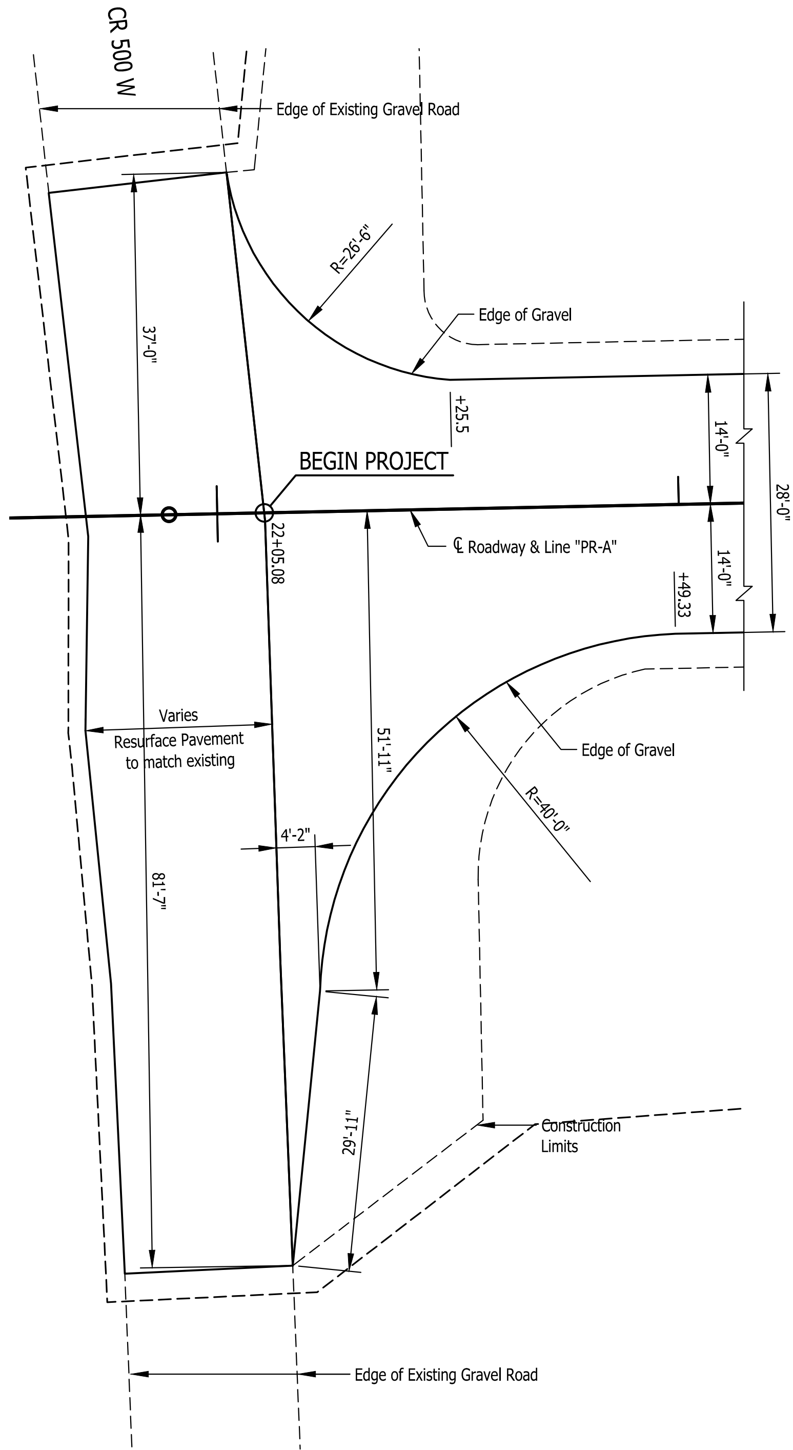
PLAN PUBLIC ROAD APPROACH Sta. 22+05.08 to Sta. 22+49.33
