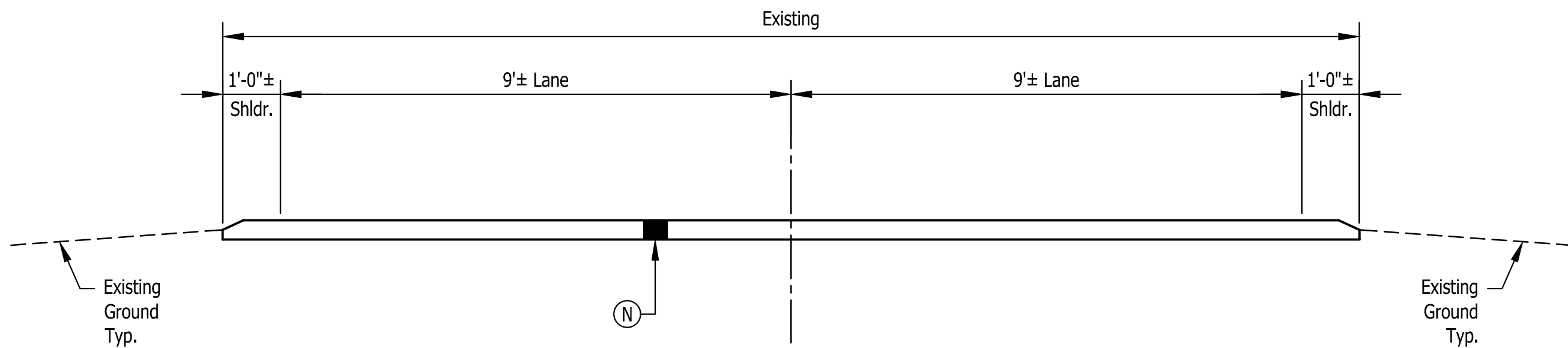
TYPICAL INCIDENTAL SECTION Sta. 25+50.83 to Sta. 26+00.83
