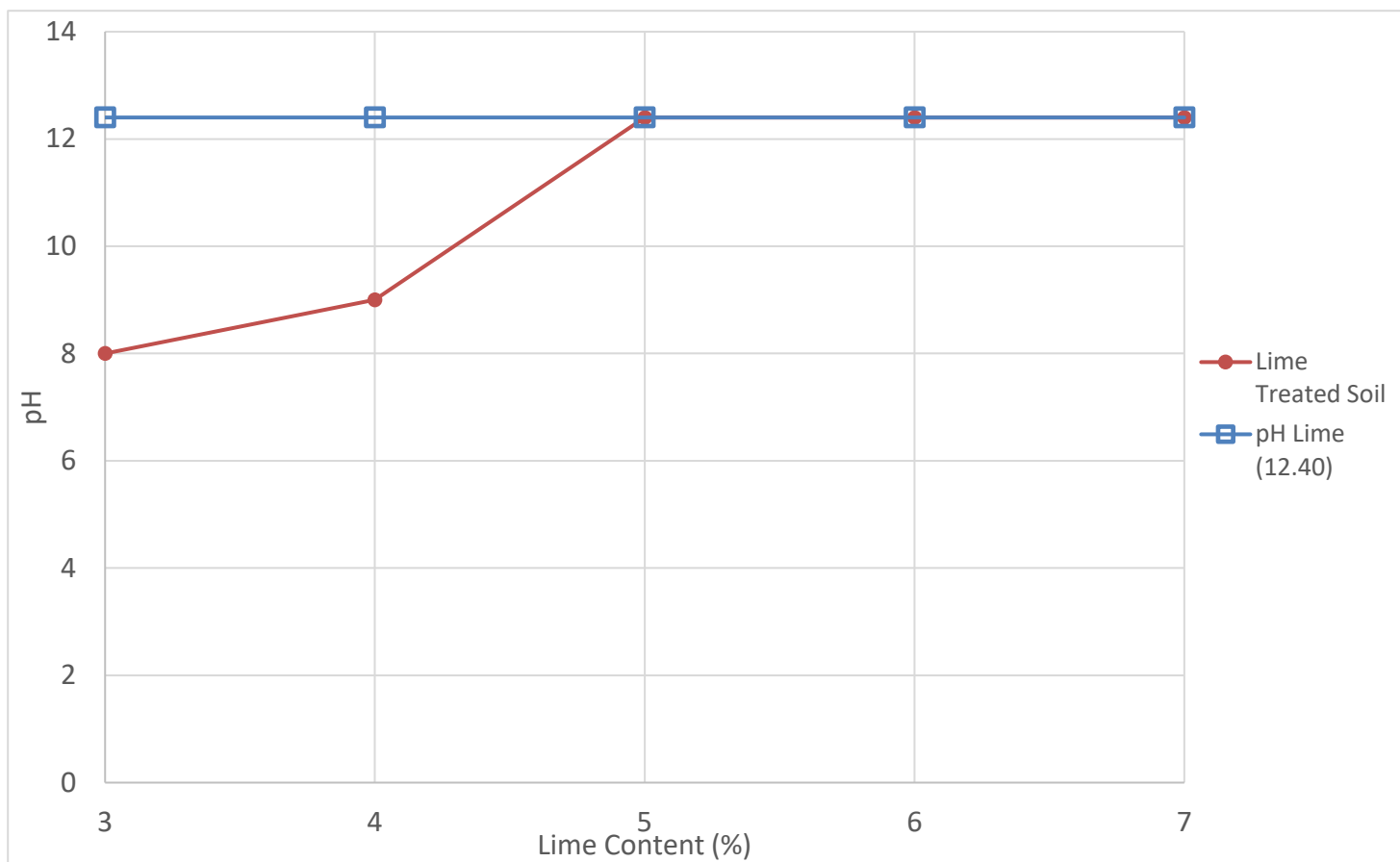
Figure 1. pH vs. Lime Content
