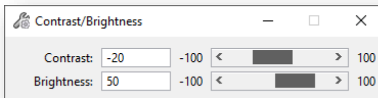
Contrast/Brightness Dialog
