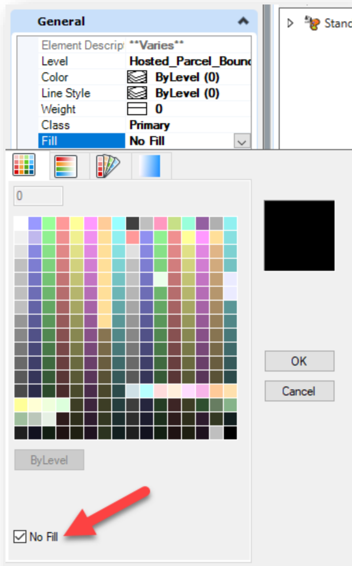
Disabling Fill
