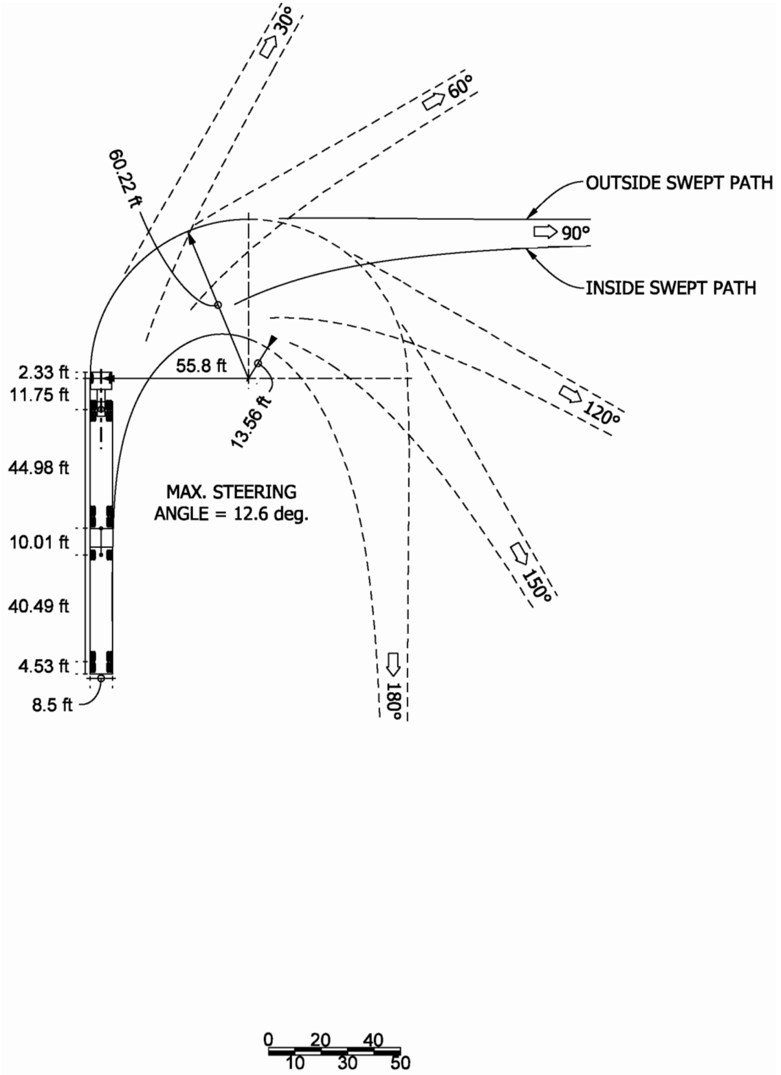
WB-109D - DESIGN VEHICLE (1" = 50' SCALE)
