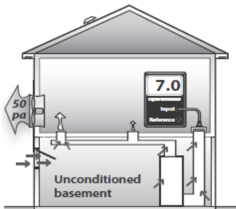
Problem return register: A pressure reading of 7 pascals indicates major air leakage near the tested register.
