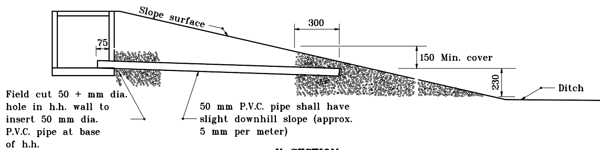
X-SECTION
