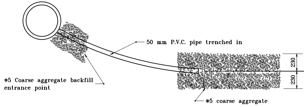
PLAN VIEW
