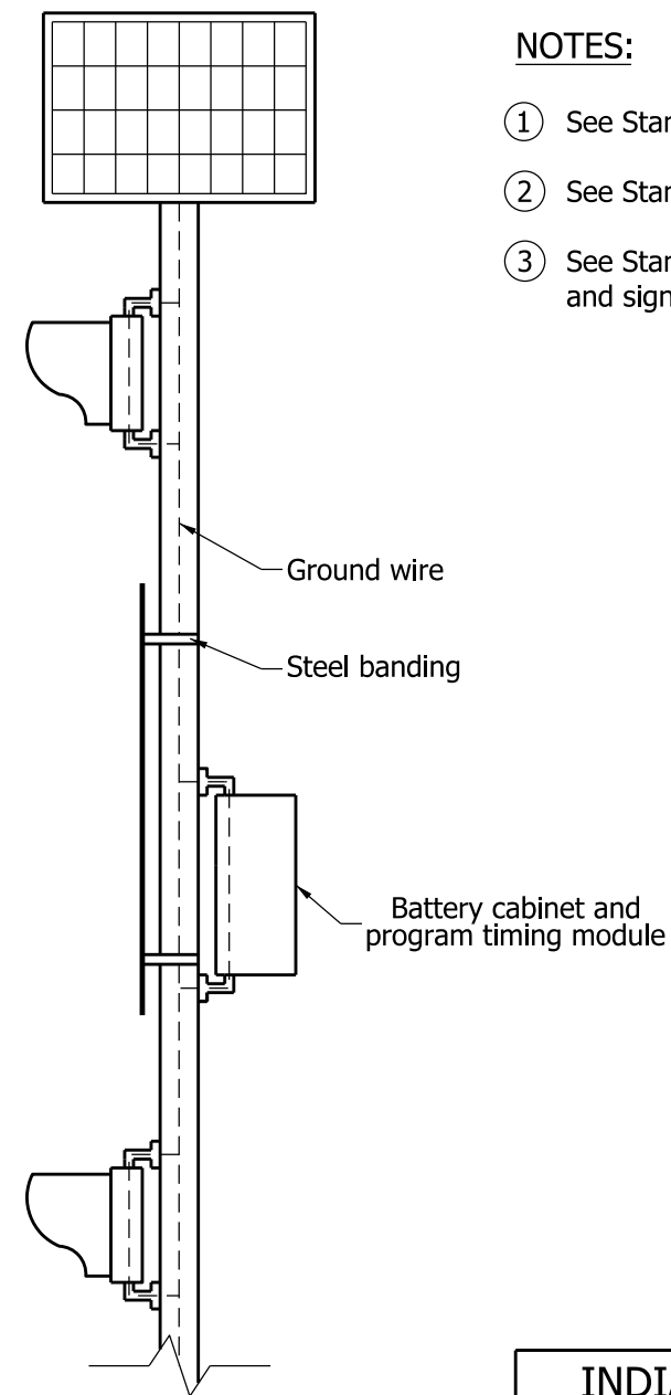
SIDE VIEW
