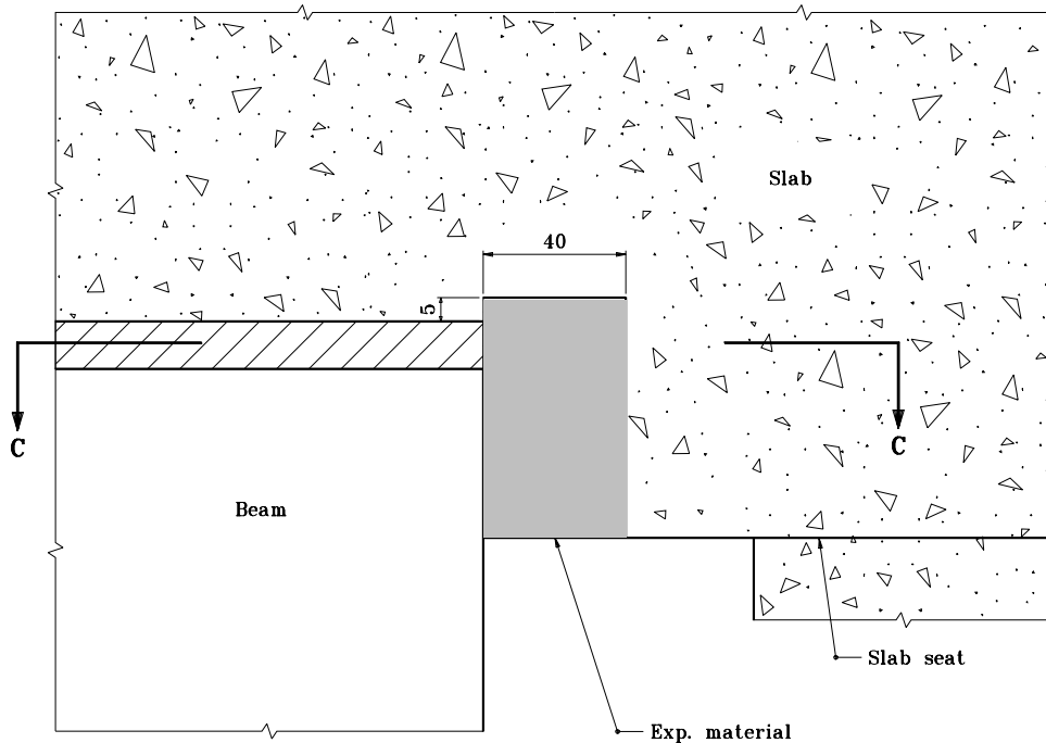
SECTION THROUGH BEAM FLANGE AND SLAB
