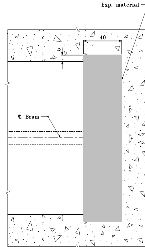
SECTION C-C
