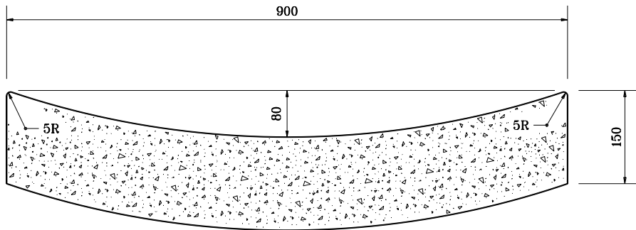
CONCRETE GUTTER
