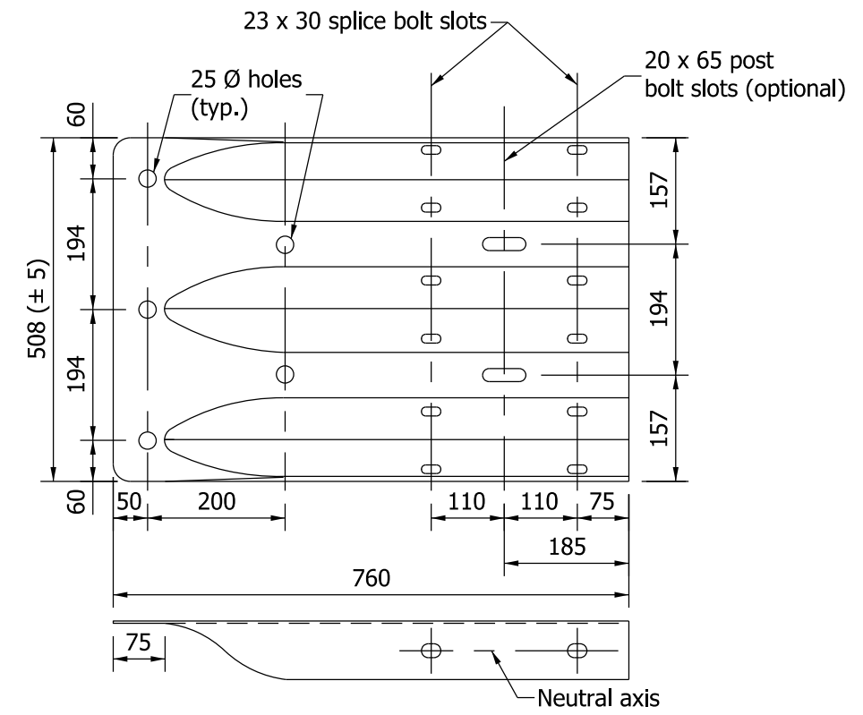
THRIE BEAM TERMINAL CONNECTOR
