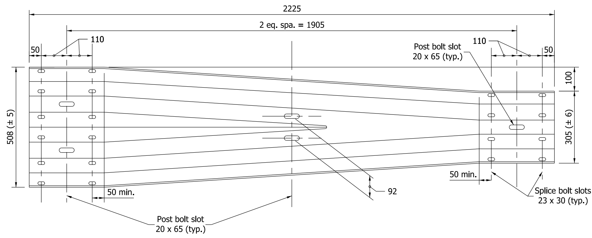
W-THRIE BEAM TRANSITION SECTION
