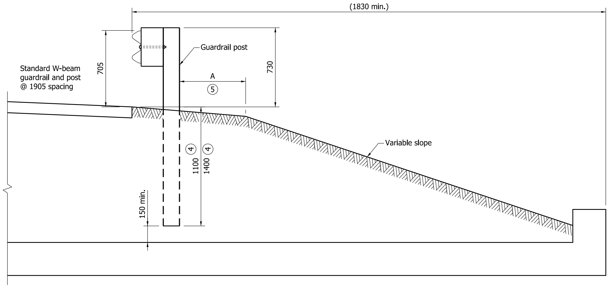
GUARDRAIL ASSEMBLY FOR COVER \geq 1250 FOR ANY STRUCTURE WIDTH
