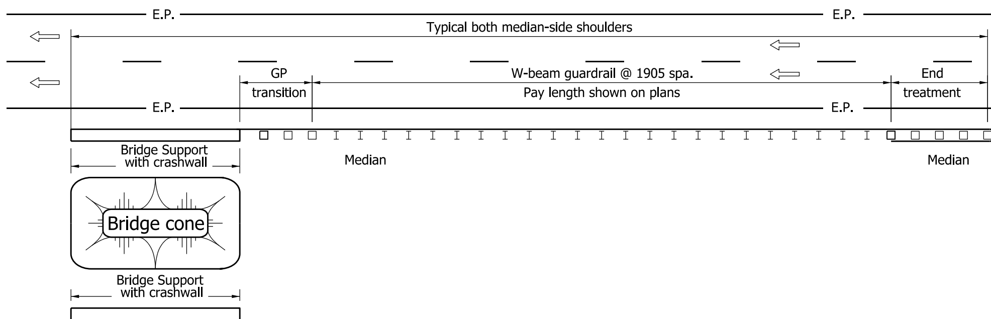
DIVIDED ROADWAY WITH TANDEM OVERHEAD STRUCTURES AND MEDIAN-SIDE BRIDGE-SUPPORT DISTANCE TO E.P. > 4900
