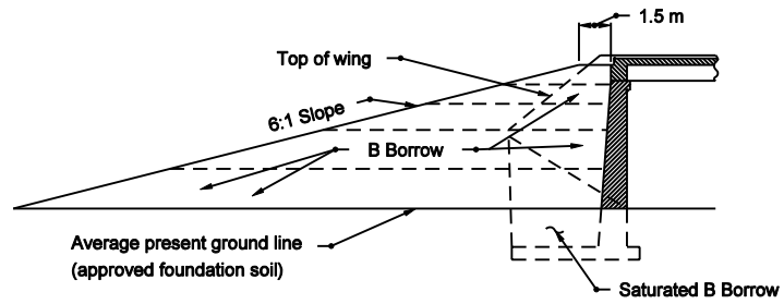
SECTION R-R
