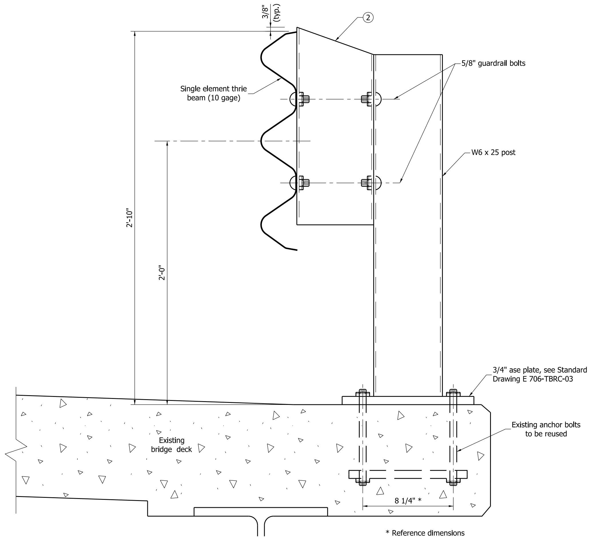
SECTION A-A BRIDGE DECK MOUNTED
