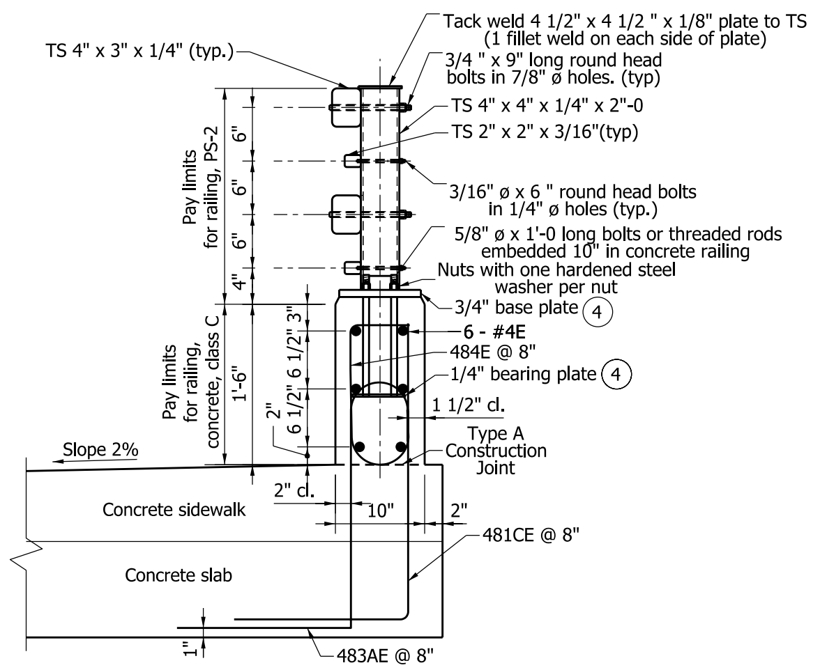
TYPICAL SECTION
