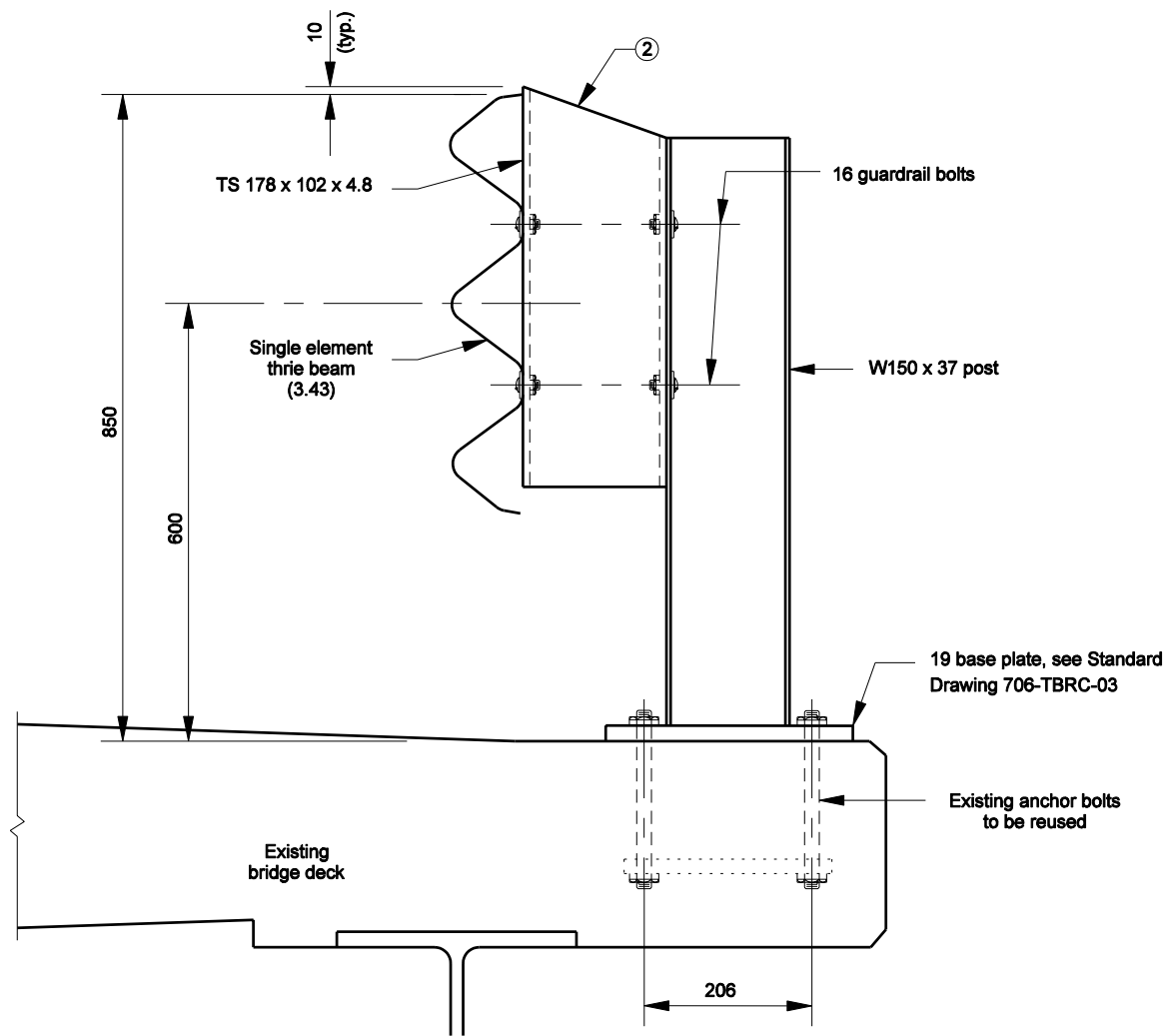
SECTION A-A BRIDGE DECK MOUNTED
