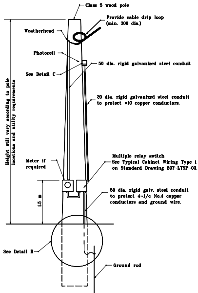
SERVICE POINT TYPE I
