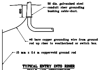
TYPICAL ENTRY INTO RISER (POLE AND STRUCTURE)
