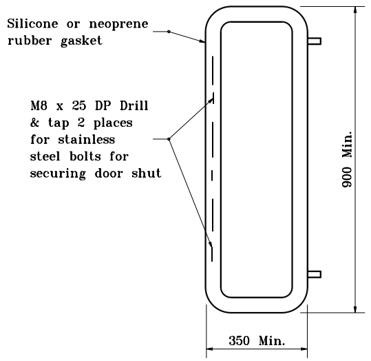
HANDHOLE FRAME DETAIL
