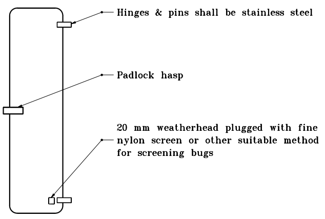
HANDHOLE COVER DETAIL
