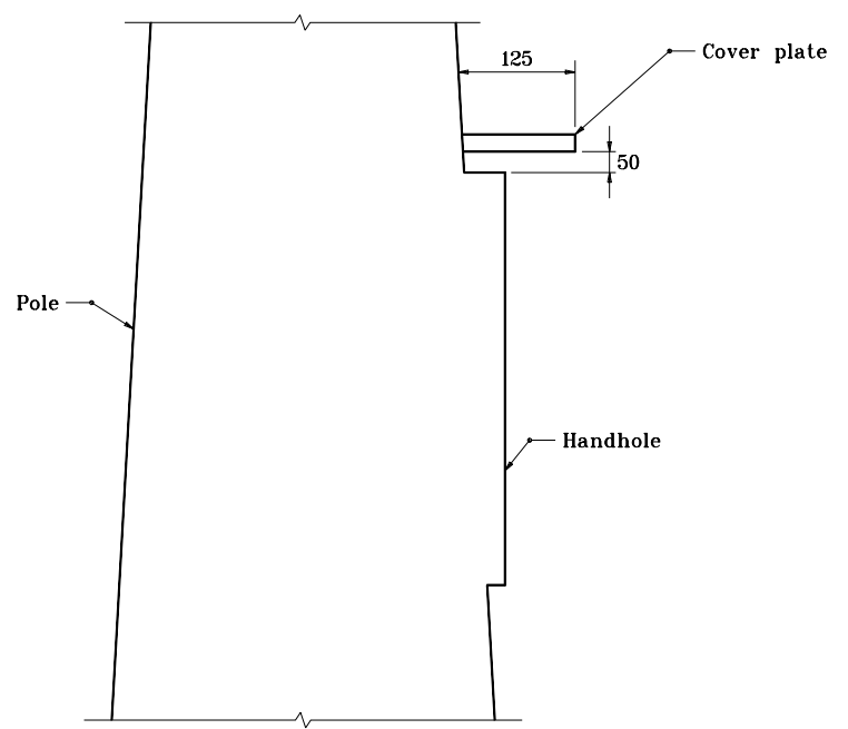
COVER PLATE
