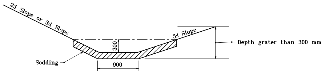
SPECIAL 900 mm BOTTOM DITCH (LOCATED BEYOND CLEAR ZONE)
