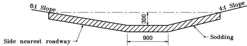
STANDARD 900 mm BOTTOM DITCH (LOCATED WITHIN CLEAR ZONE)
