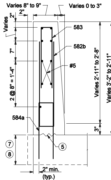
SECTION C-C
