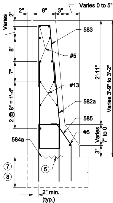
SECTION B-B
