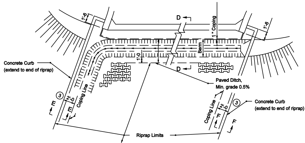
FLARED WINGS
