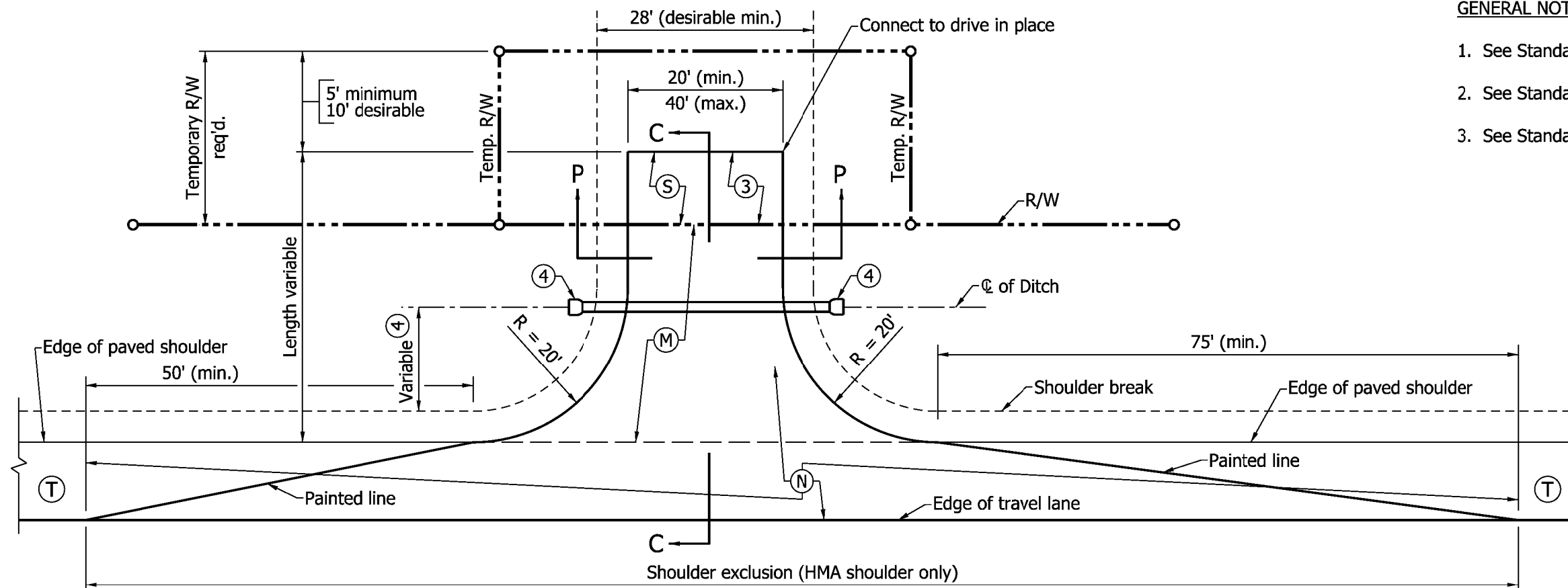
PLAN VIEW (PAVED SHOULDER 8 FEET OR GREATER IN WIDTH)
