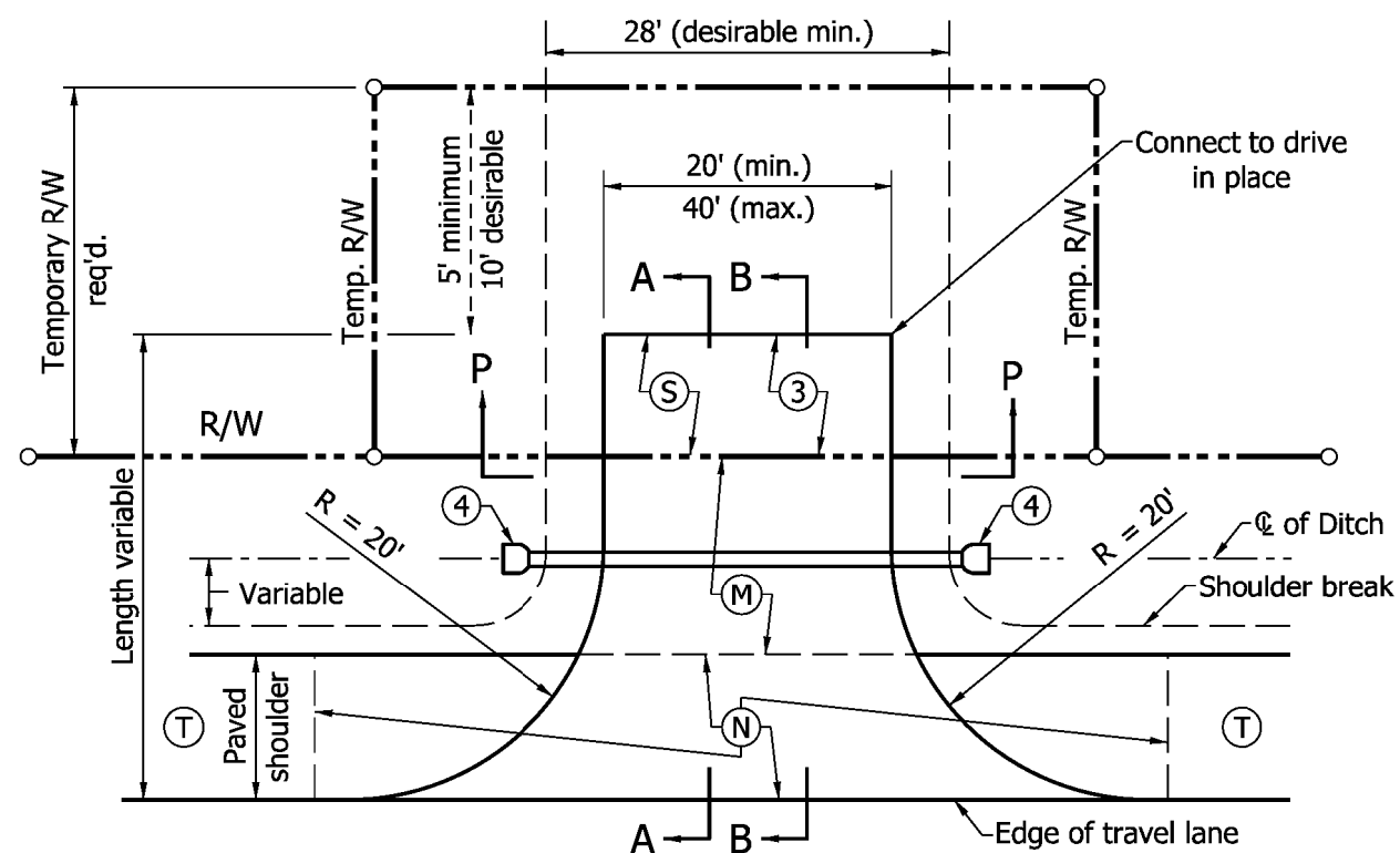
PLAN VIEW (PAVED SHOULDER LESS THAN 8 FEET IN WIDTH OR UNPAVED SHOULDER)
