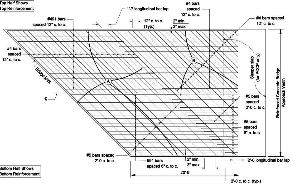
REINFORCEMENT DETAIL FOR SKEWED APPROACH
