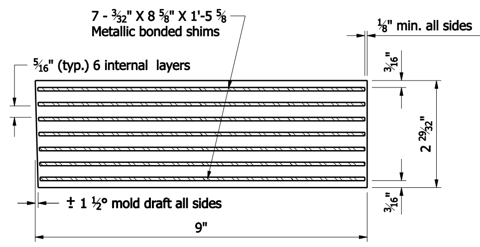
SECTION C-C TYPE 3
