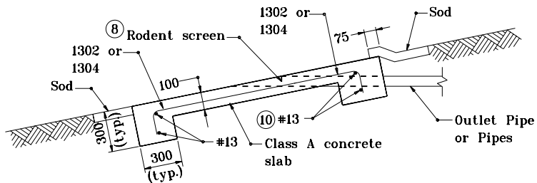
TYPICAL SECTION
