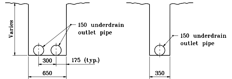
TWIN OUTLET DETAIL
