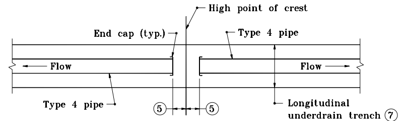
PLAN-INSTALLATION AT CREST
