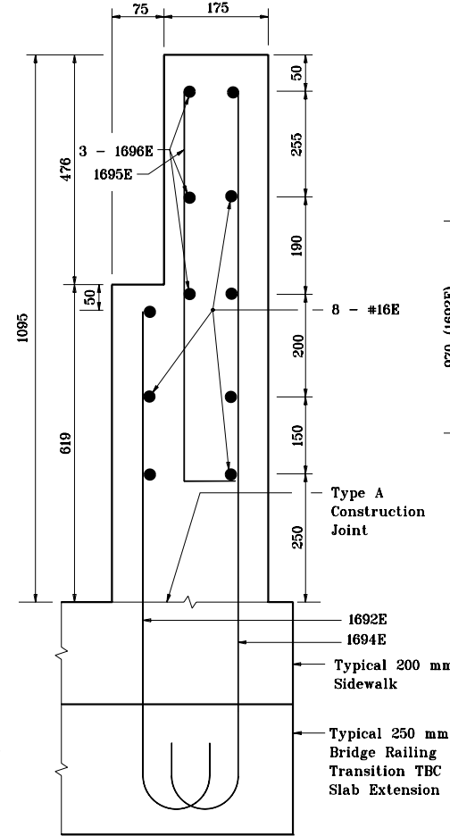
Section C - C
