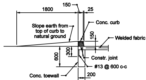
SECTION C-C
