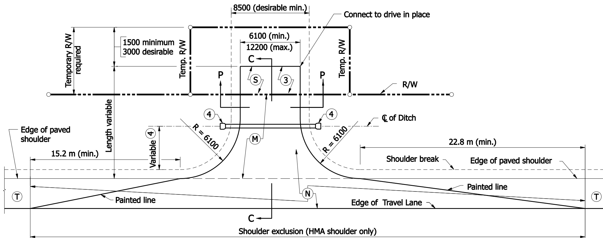
PLAN VIEW (PAVED SHOULDER 2400 OR GREATER IN WIDTH)
