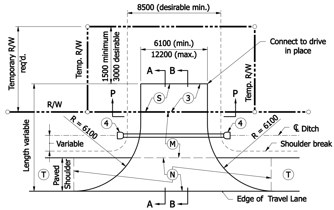
PLAN VIEW (PAVED SHOULDER LESS THAN 2400 IN WIDTH OR UNPAVED SHOULDER)
