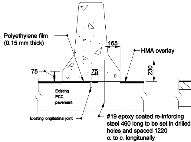
840 HEIGHT CONCRETE BARRIER WALL
