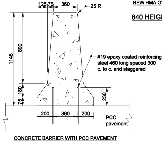
1145 HEIGHT CONCRETE BARRIER WALL
