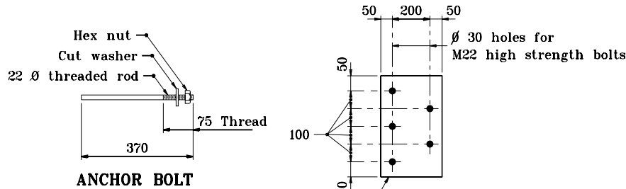
ANCHOR BOLT
