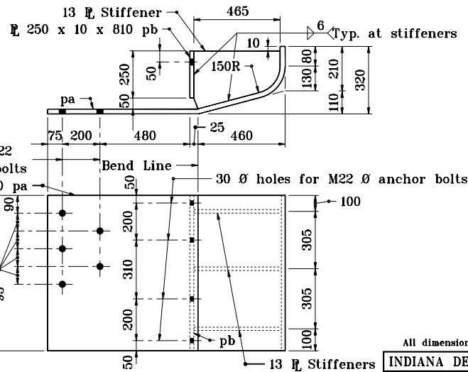
DETAIL OF NOSE DEFLECTOR - SQUARE
