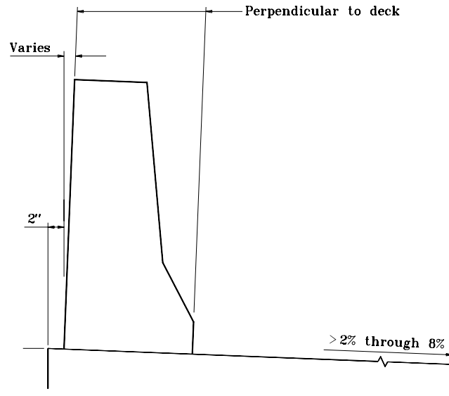
Superelevated Section
