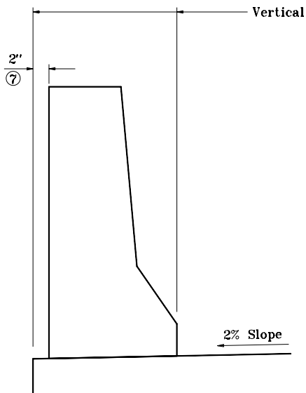
Crown Section
