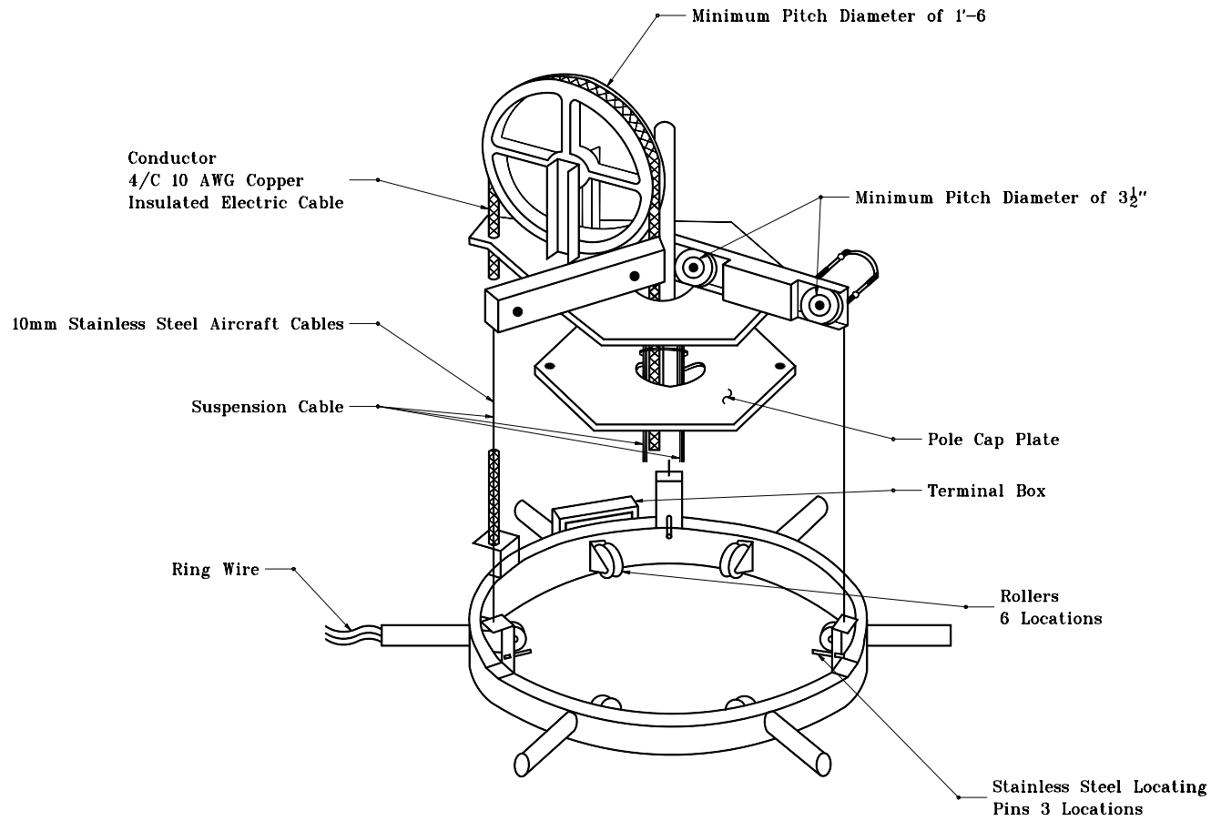
RING ASSEMBLY
