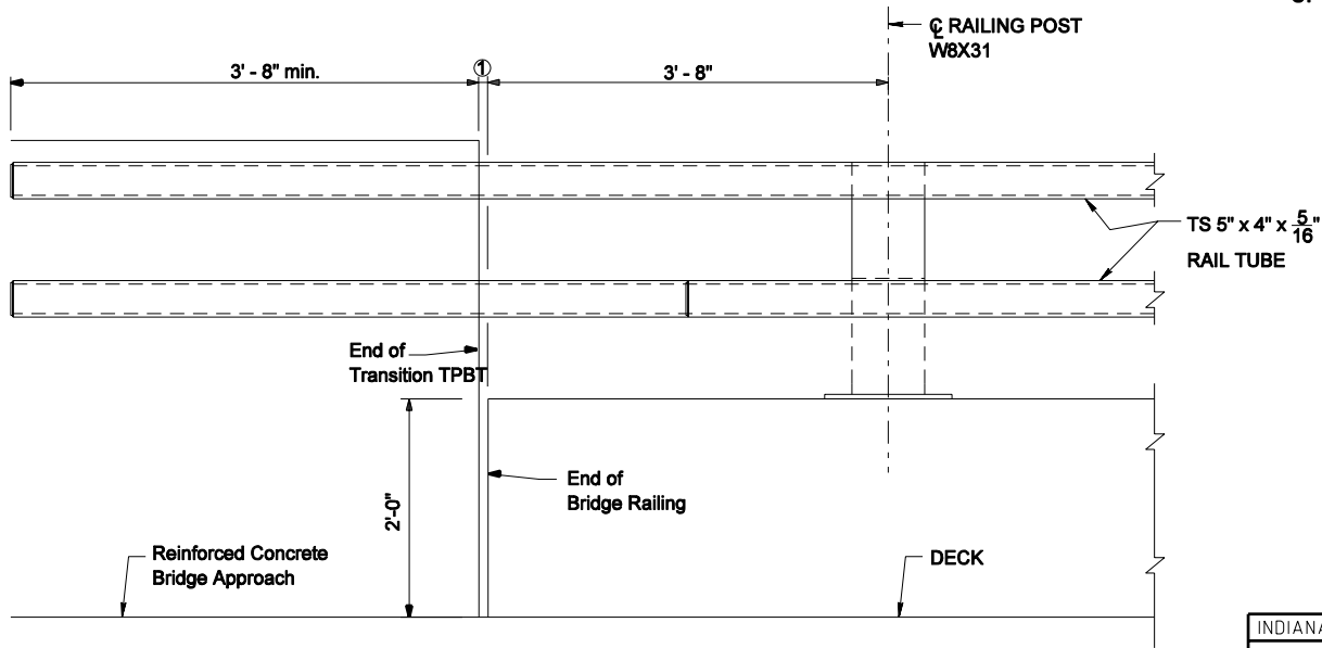
RAILING ELEVATION AT ENDS
