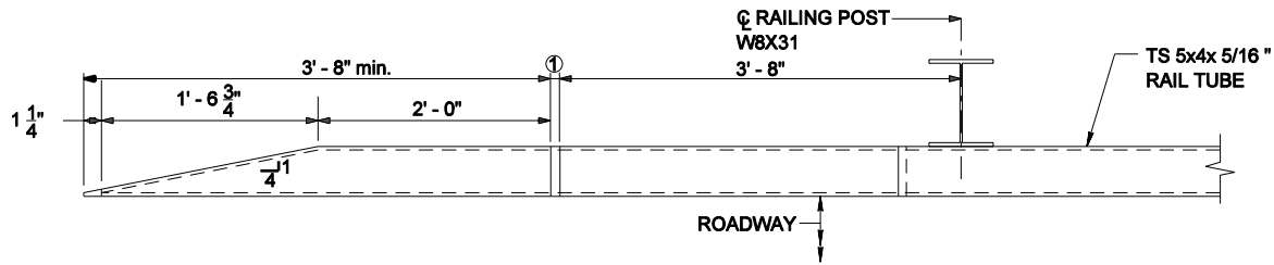
TOP VIEW (CONCRETE RAILING NOT SHOWN)
