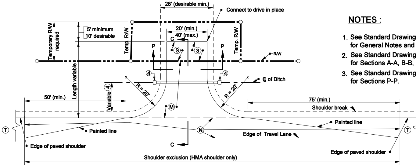
PLAN VIEW (PAVED SHOULDER 8 FEET OR GREATER IN WIDTH)
