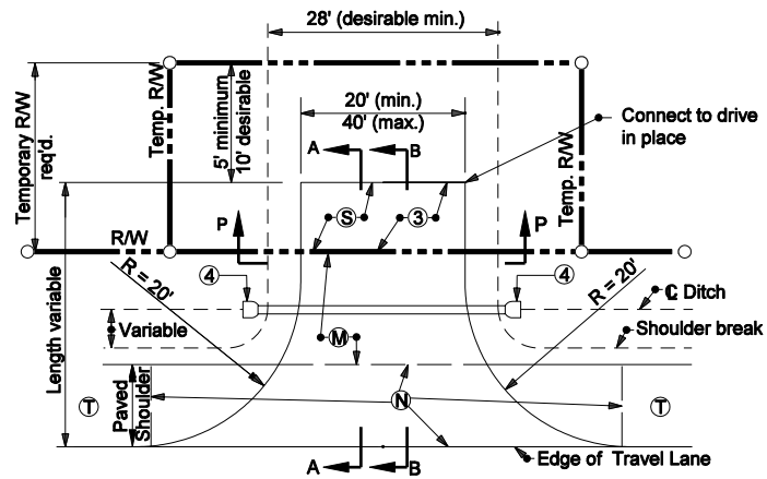
PLAN VIEW (PAVED SHOULDER LESS THAN 8 FEET IN WIDTH OR UNPAVED SHOULDER)
