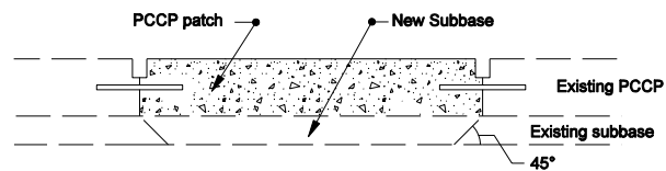
SECTION A-A Where Existing Subbase must be removed
