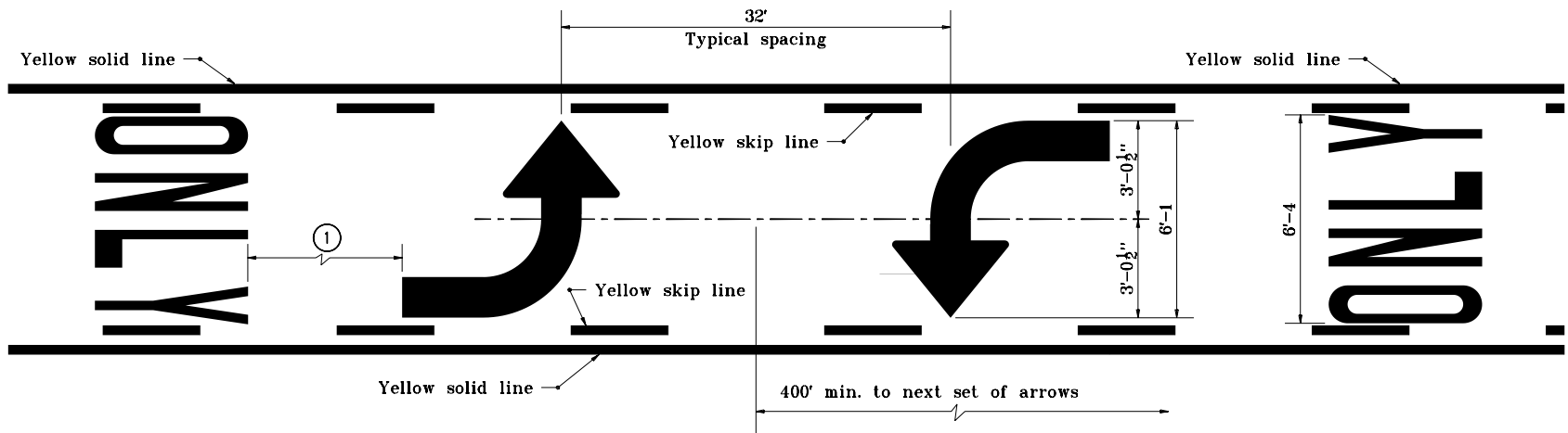
PAVEMENT MARKING FOR BI-DIRECTIONAL LEFT TURN LANE (WORD AND SYMBOL MARKINGS)
