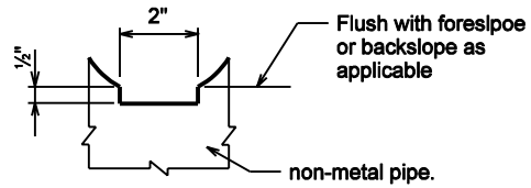
DRAINAGE NOTCH
