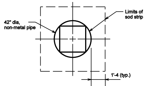
PLAN, SQUARE FOUNDATION
