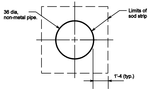
PLAN, ROUND FOUNDATION
