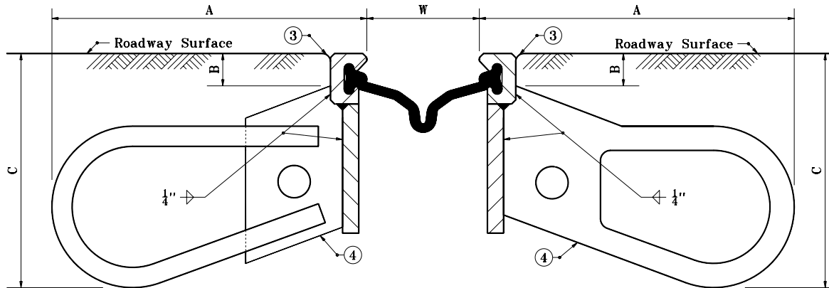
INSTALLATION DETAIL
