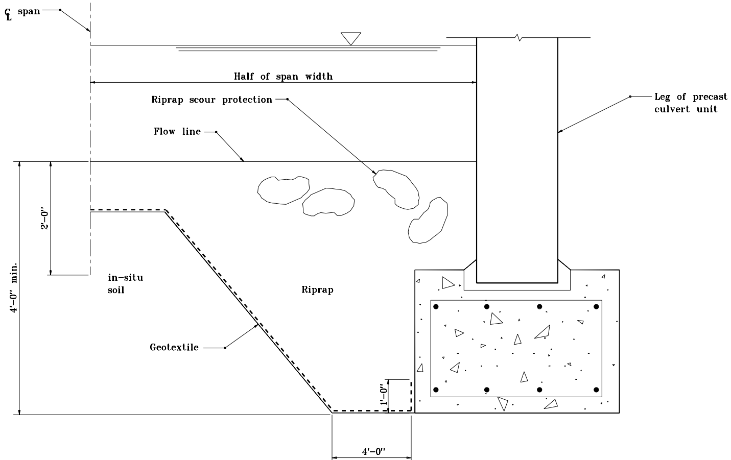
SECTION A-A RIPRAP METHOD For Span Width of 20'-0" or Greater.
