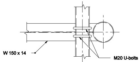
LOWER CHORD CONNECTION DETAIL
