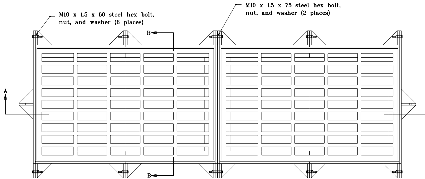
PLAN
