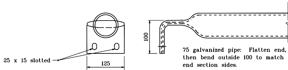
TRANSVERSE SAFETY BAR DETAILS
